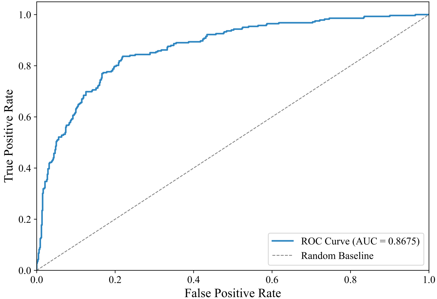
ROC Curve — ENGLISH_MANUAL (paraphrase-multilingual-mpnet-base-v2, XGBoost_Optimized)
