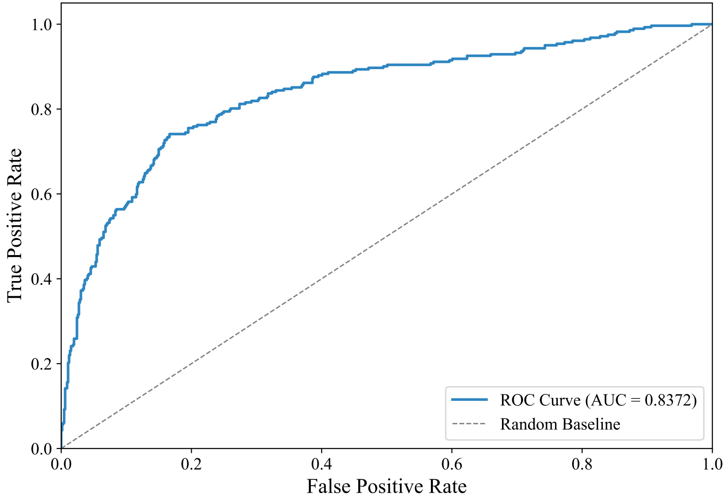
ROC Curve — ENGLISH_MANUAL (upskyy/bge-m3-korean, Random_Forest_Optimized)
