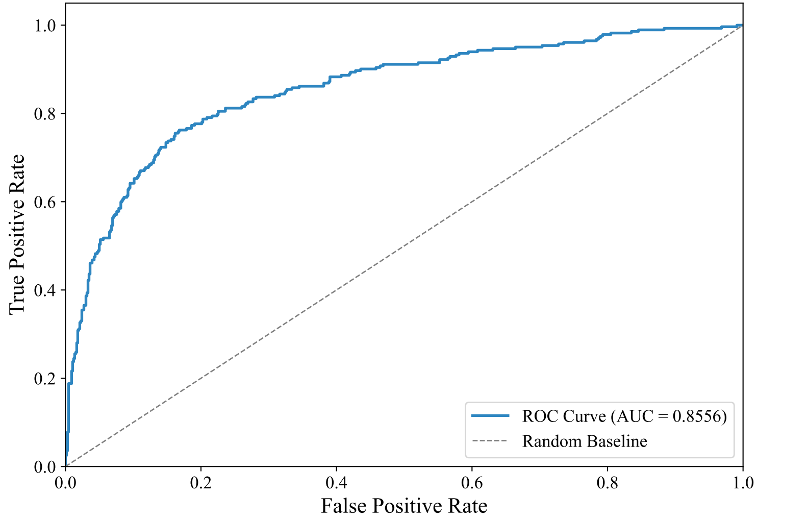
ROC Curve — ENGLISH_MANUAL (upskyy/bge-m3-korean, XGBoost_Optimized)
