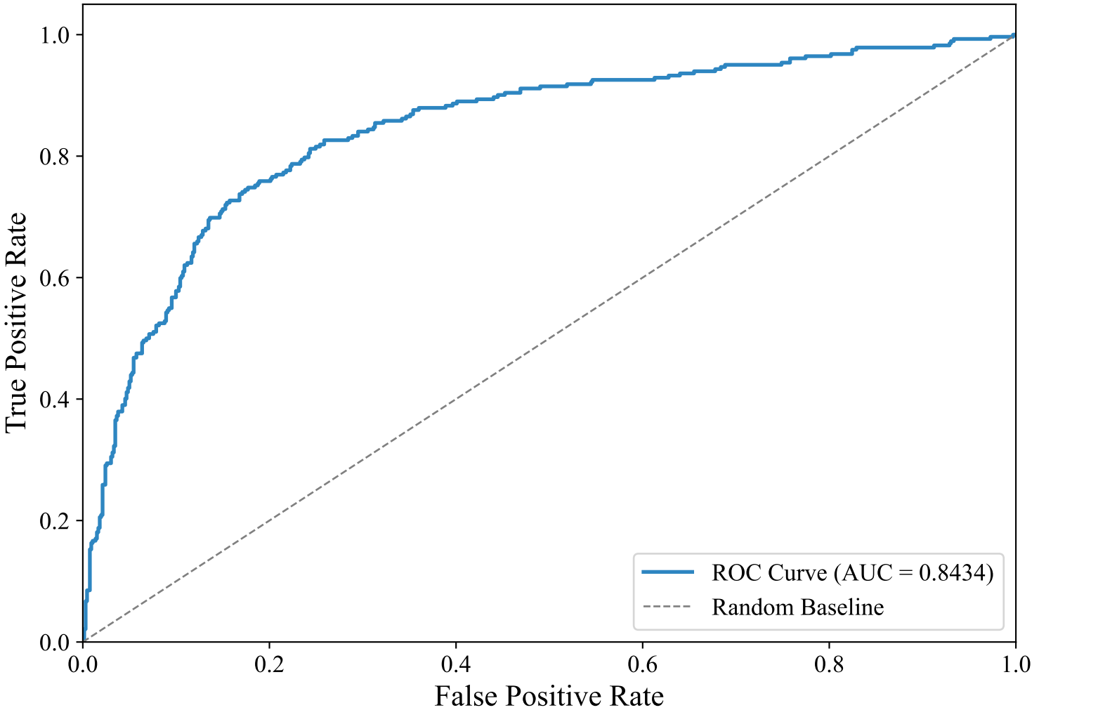
ROC Curve — ENGLISH_MANUAL (xlm-roberta-base, Voting_Ensemble)
