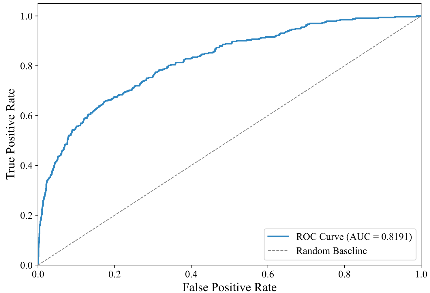
ROC Curve — GERMAN_MANUAL (bert-base-multilingual-uncased, LightGBM_Optimized)
