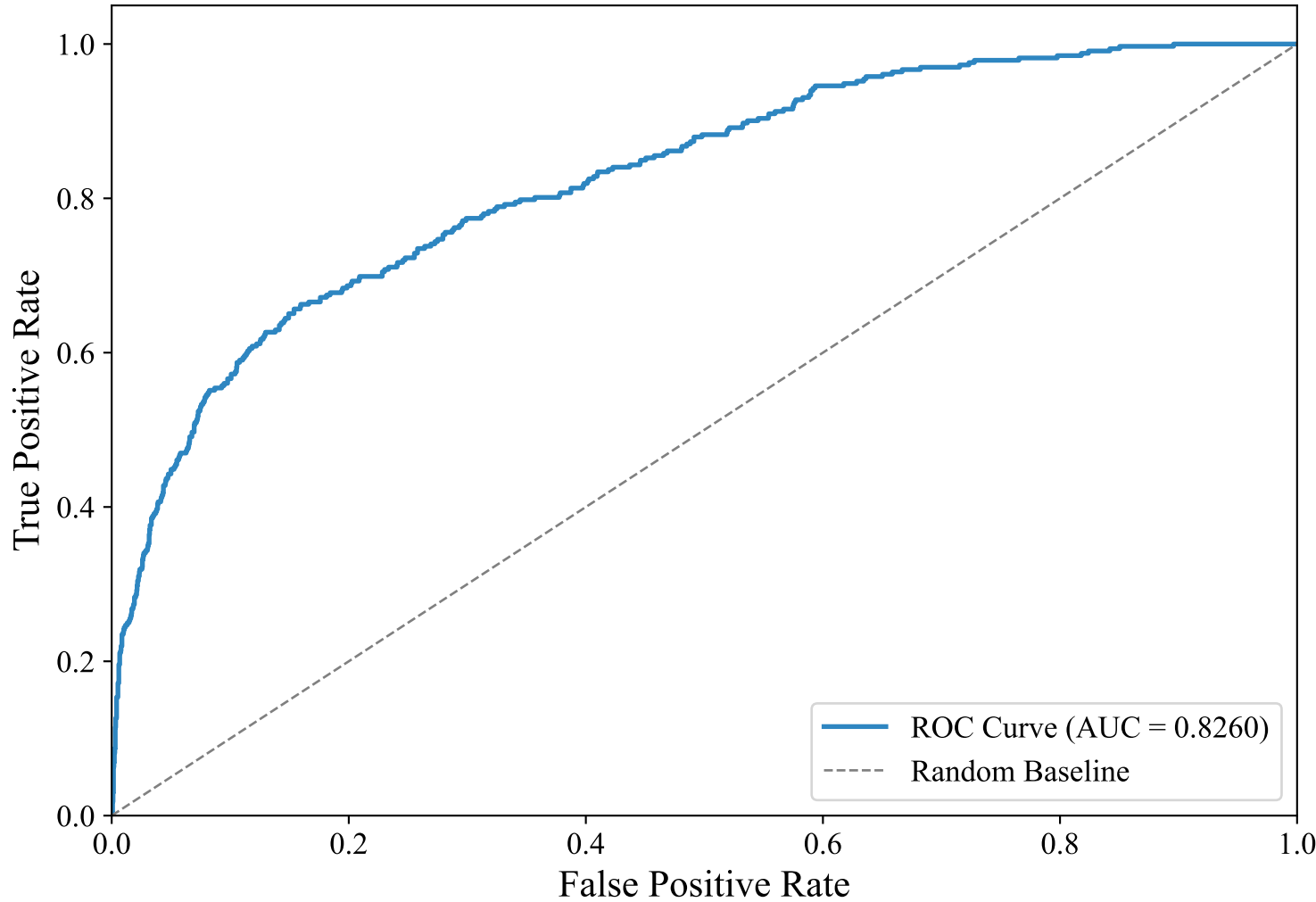
ROC Curve — GERMAN_MANUAL (bert-base-multilingual-uncased, Voting_Ensemble)
