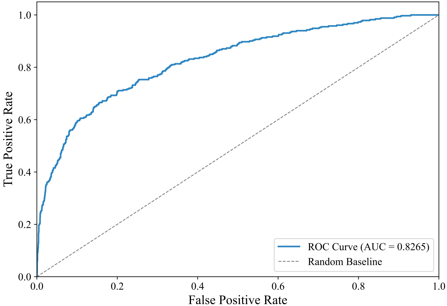
ROC Curve — GERMAN_MANUAL (bert-base-multilingual-uncased, XGBoost)
