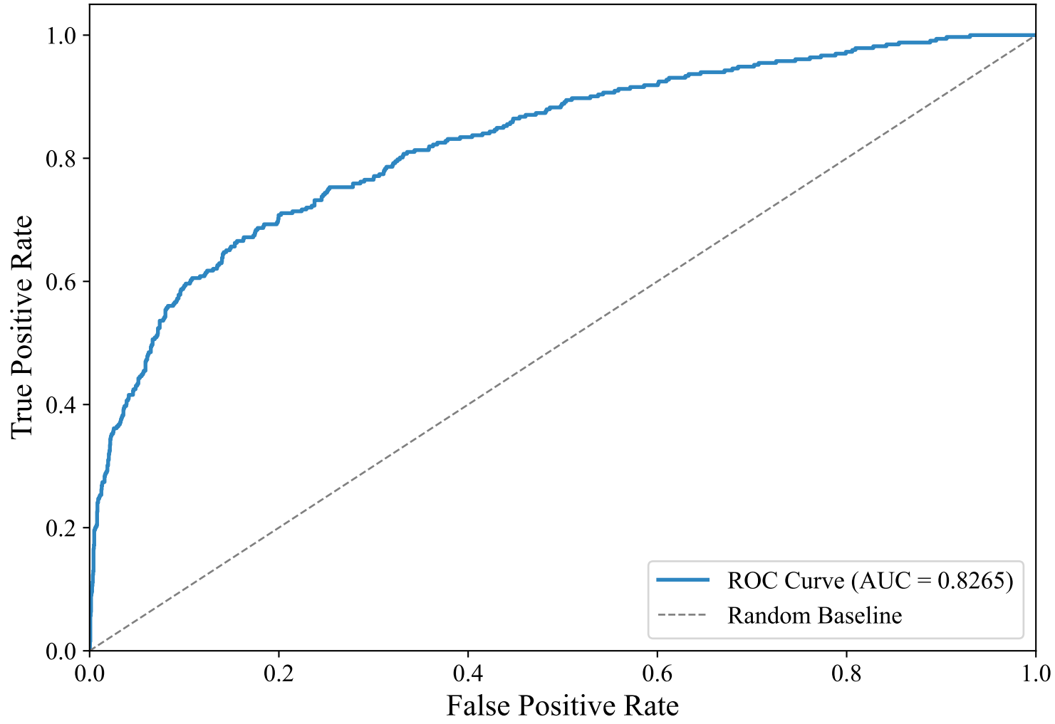
ROC Curve — GERMAN_MANUAL (bert-base-multilingual-uncased, XGBoost_Optimized)
