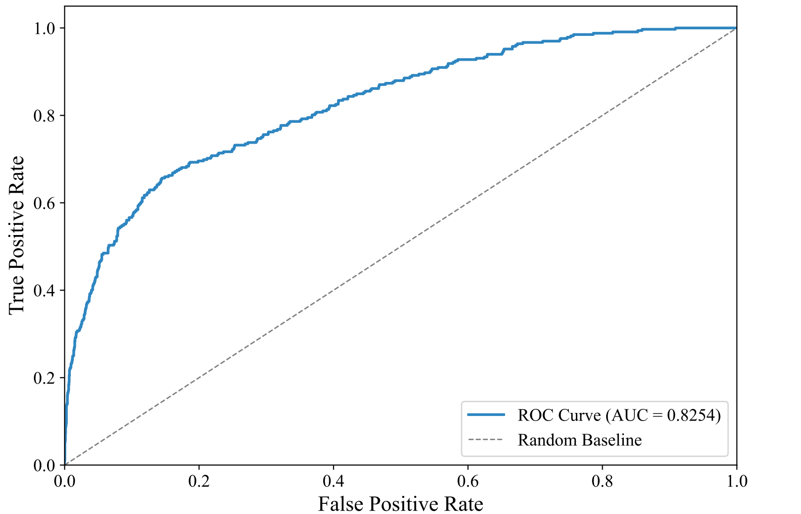
ROC Curve — GERMAN_MANUAL (efederici/e5-base-multilingual-4096, XGBoost_Optimized)
