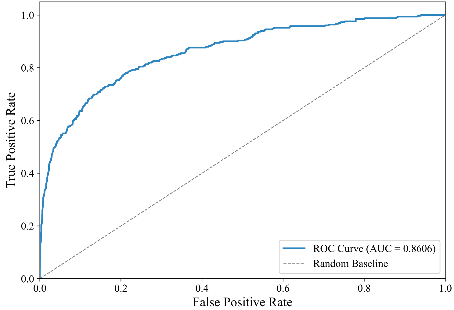
ROC Curve — GERMAN_MANUAL (intfloat/multilingual-e5-large-instruct, Voting_Ensemble)
