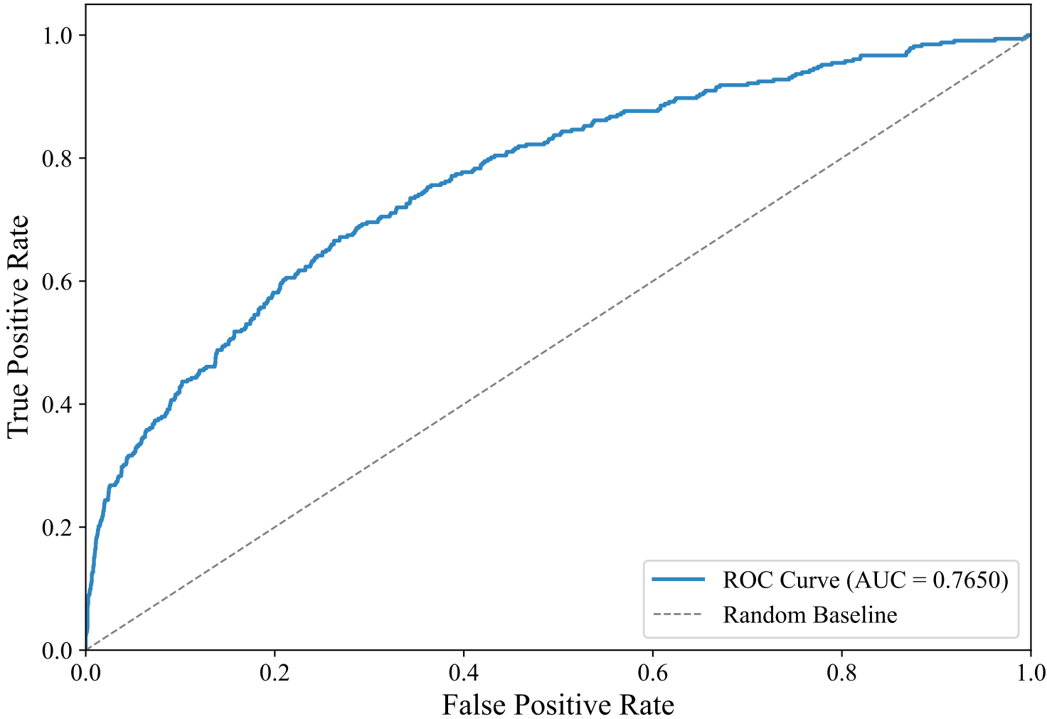
ROC Curve — GERMAN_MANUAL (paraphrase-multilingual-MiniLM-L12-v2, LightGBM)
