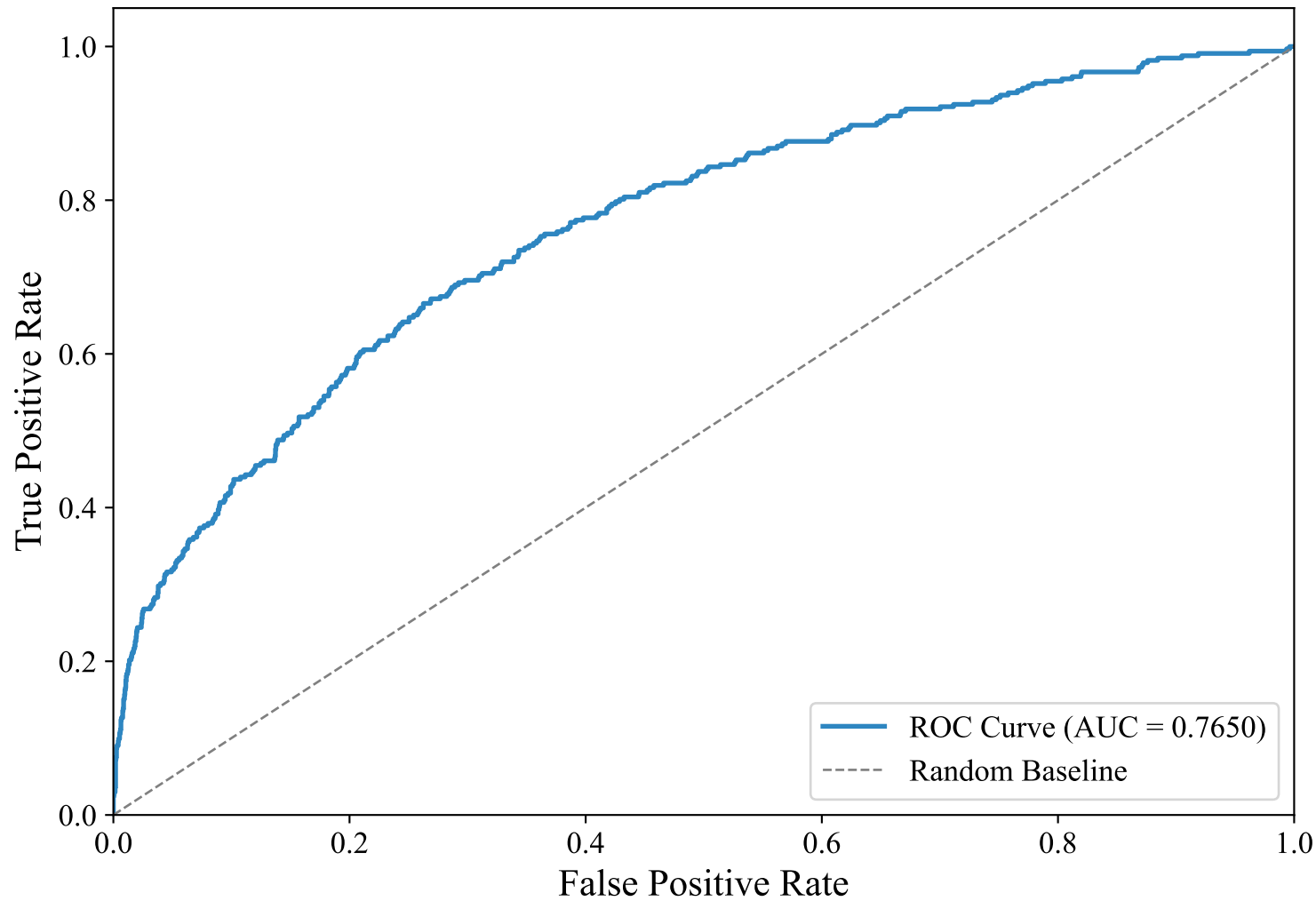
ROC Curve — GERMAN_MANUAL (paraphrase-multilingual-MiniLM-L12-v2, LightGBM_Optimized)
