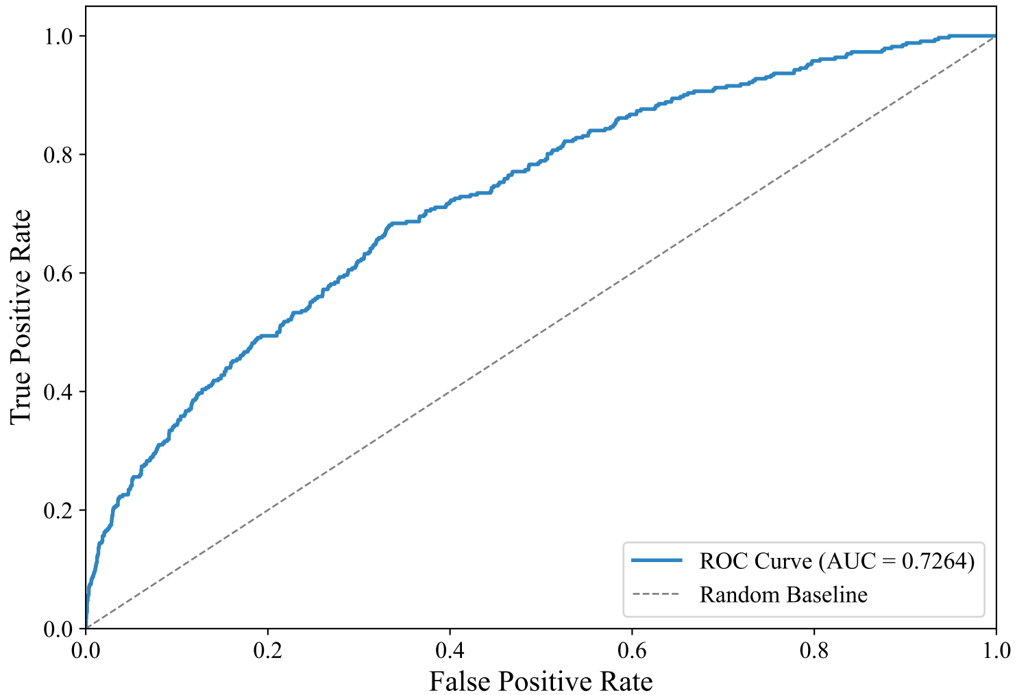
ROC Curve — GERMAN_MANUAL (paraphrase-multilingual-MiniLM-L12-v2, Random_Forest_Optimized)
