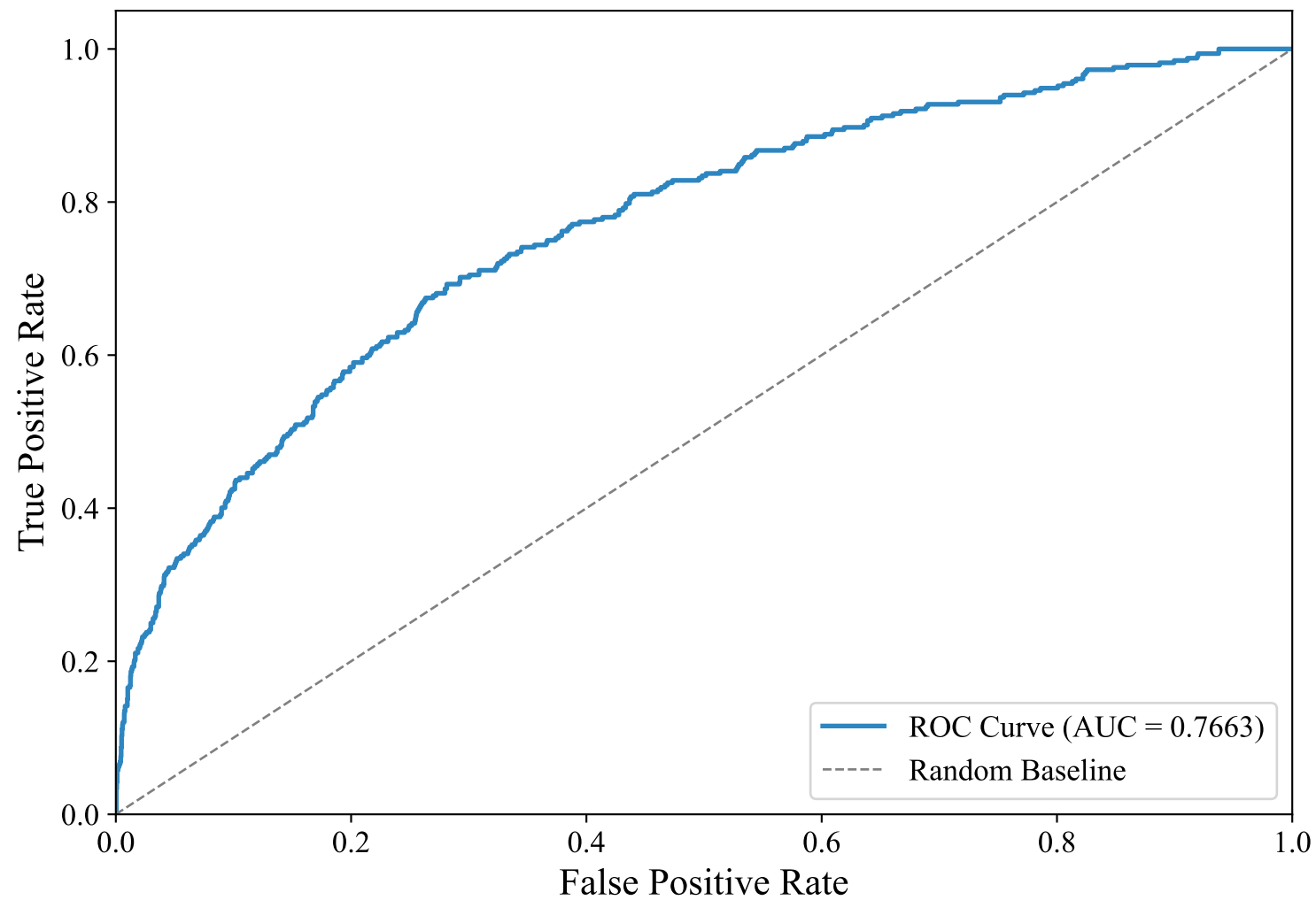
ROC Curve — GERMAN_MANUAL (paraphrase-multilingual-MiniLM-L12-v2, Voting_Ensemble)
