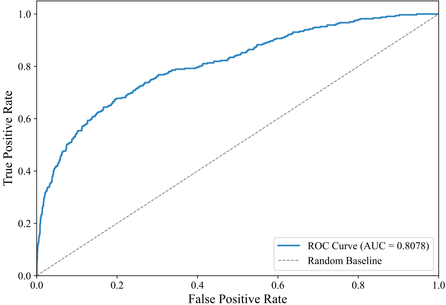
ROC Curve — GERMAN_MANUAL (paraphrase-multilingual-mpnet-base-v2, LightGBM_Optimized)
