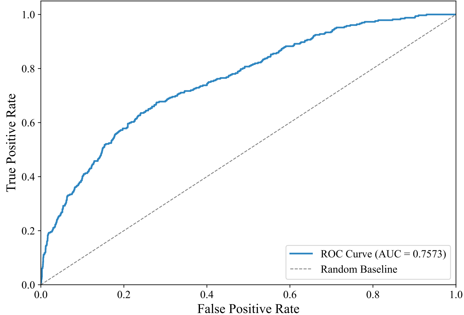
ROC Curve — GERMAN_MANUAL (paraphrase-multilingual-mpnet-base-v2, Random_Forest_Optimized)
