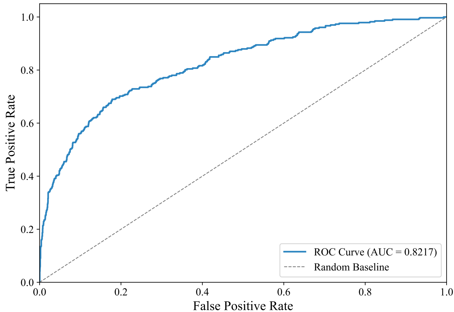
ROC Curve — GERMAN_MANUAL (paraphrase-multilingual-mpnet-base-v2, XGBoost)
