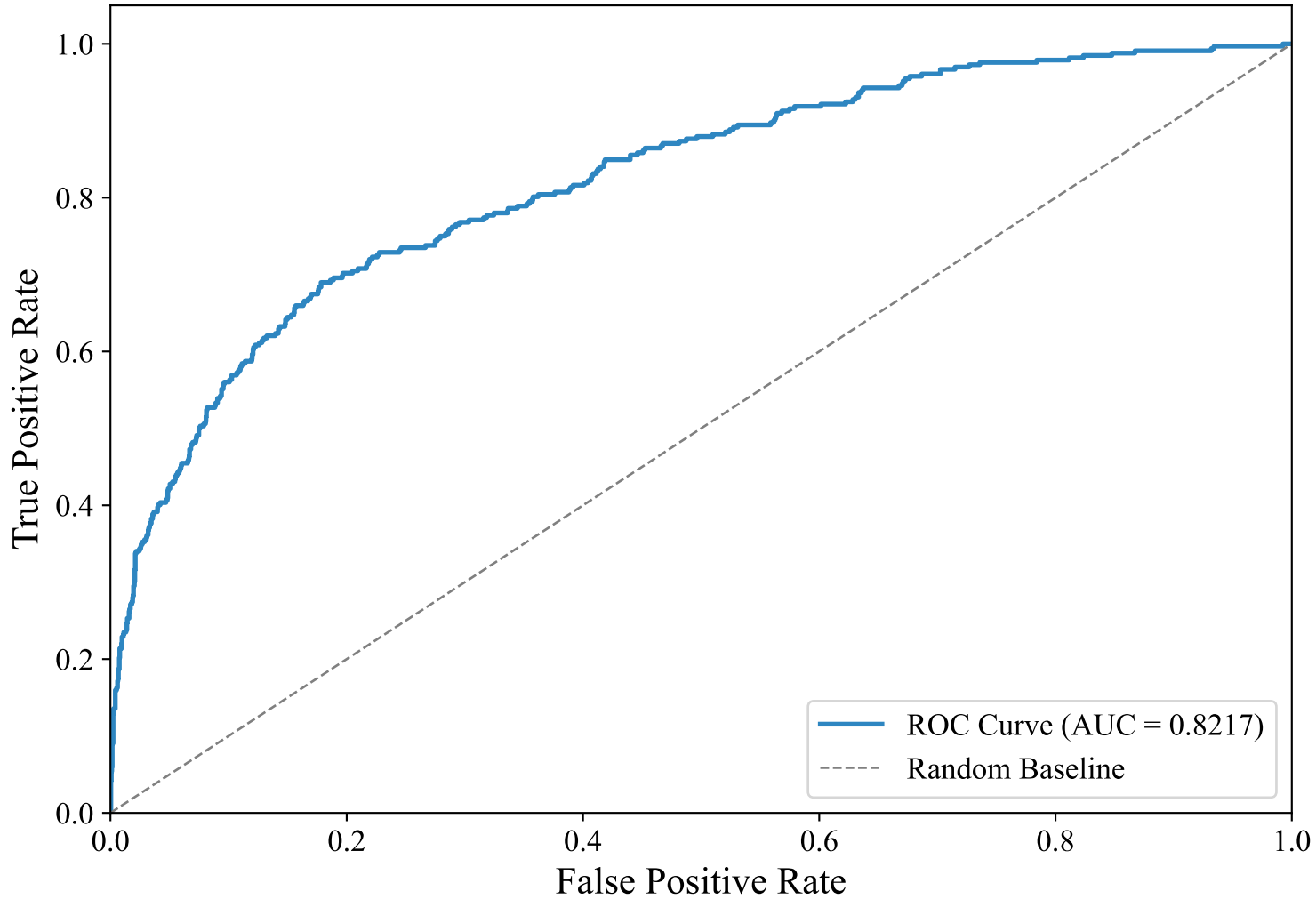
ROC Curve — GERMAN_MANUAL (paraphrase-multilingual-mpnet-base-v2, XGBoost_Optimized)
