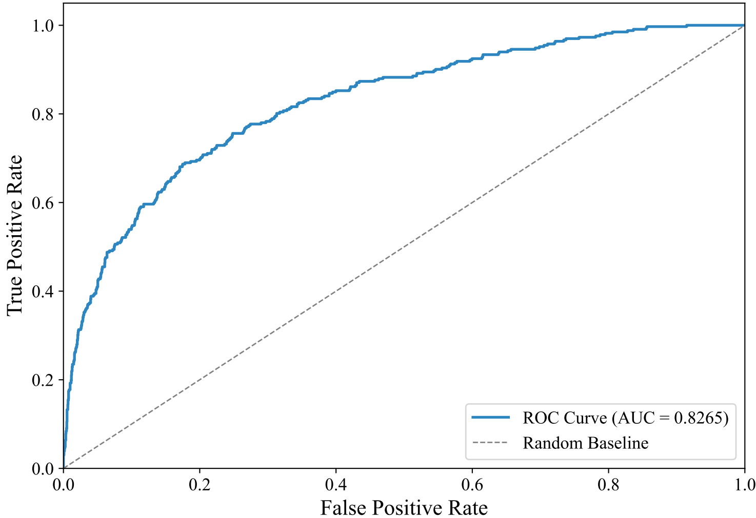
ROC Curve — GERMAN_MANUAL (snowflake-arctic-embed-l-v2.0, Random_Forest)
