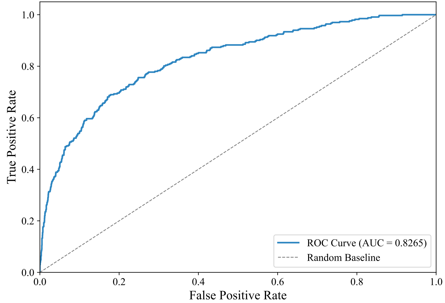
ROC Curve — GERMAN_MANUAL (snowflake-arctic-embed-l-v2.0, Random_Forest_Optimized)
