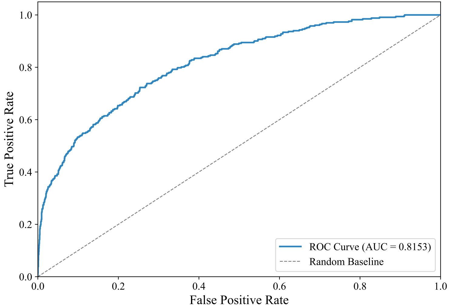
ROC Curve — GERMAN_MANUAL (upskyy/bge-m3-korean, Random_Forest_Optimized)
