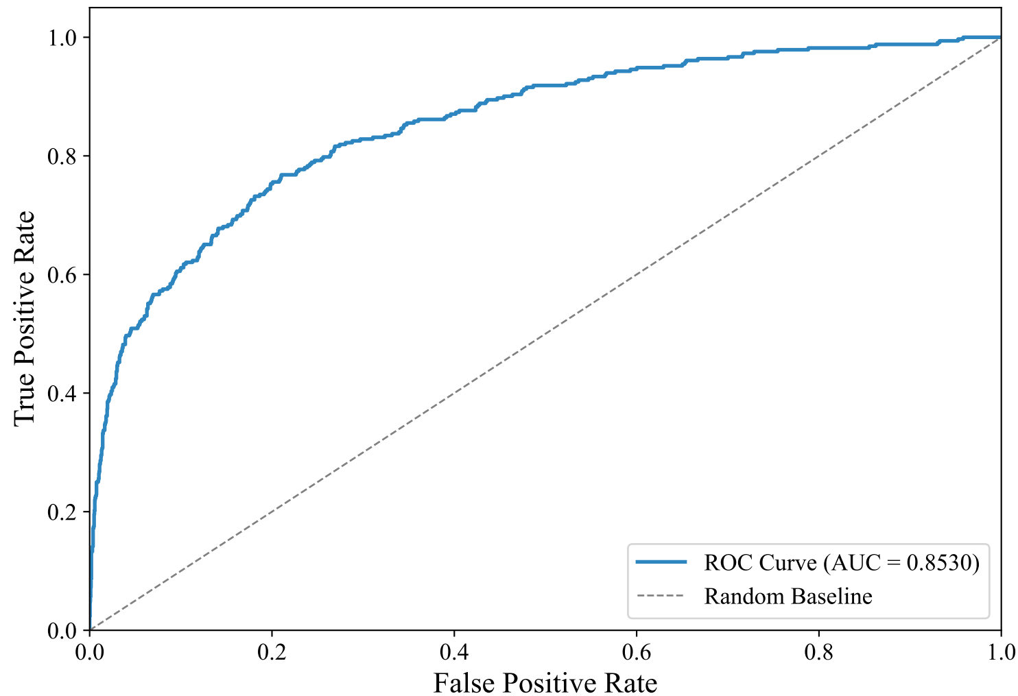
ROC Curve — GERMAN_MANUAL (upskyy/bge-m3-korean, XGBoost)
