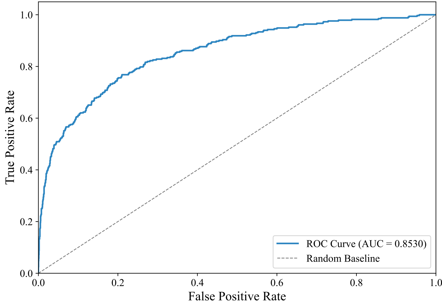
ROC Curve — GERMAN_MANUAL (upskyy/bge-m3-korean, XGBoost_Optimized)
