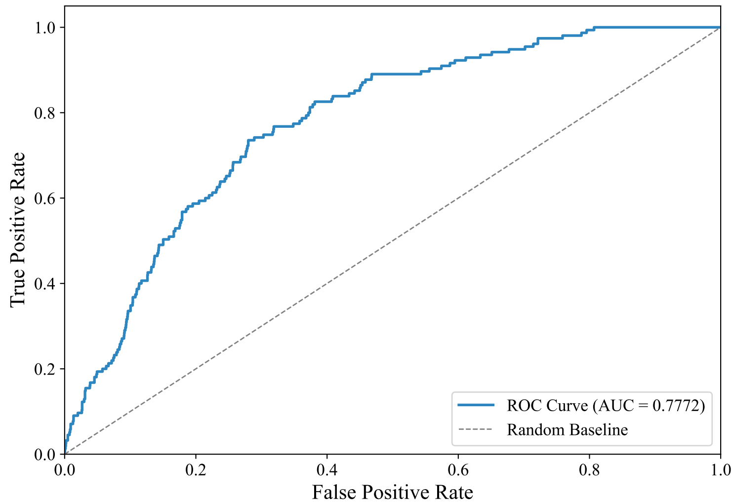
ROC Curve — SWEDISH_MANUAL (efederici/e5-base-multilingual-4096, Random_Forest)
