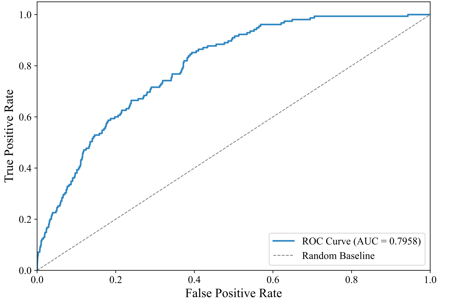
ROC Curve — SWEDISH_MANUAL (efederici/e5-base-multilingual-4096, XGBoost)
