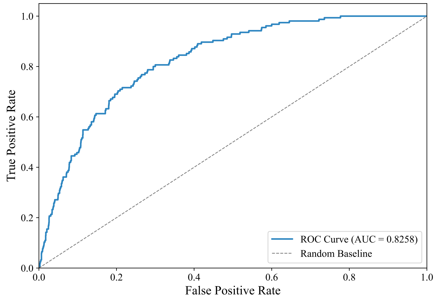
ROC Curve — SWEDISH_MANUAL (intfloat/multilingual-e5-large-instruct, Voting_Ensemble)
