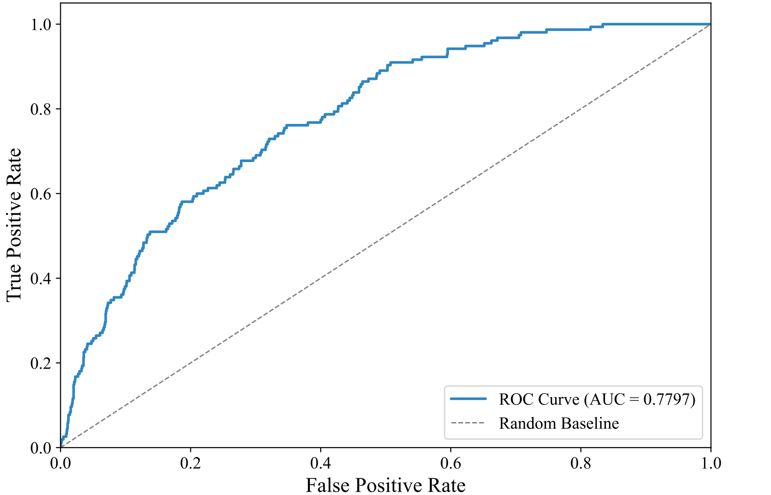
ROC Curve — SWEDISH_MANUAL (paraphrase-multilingual-MiniLM-L12-v2, Voting_Ensemble)
