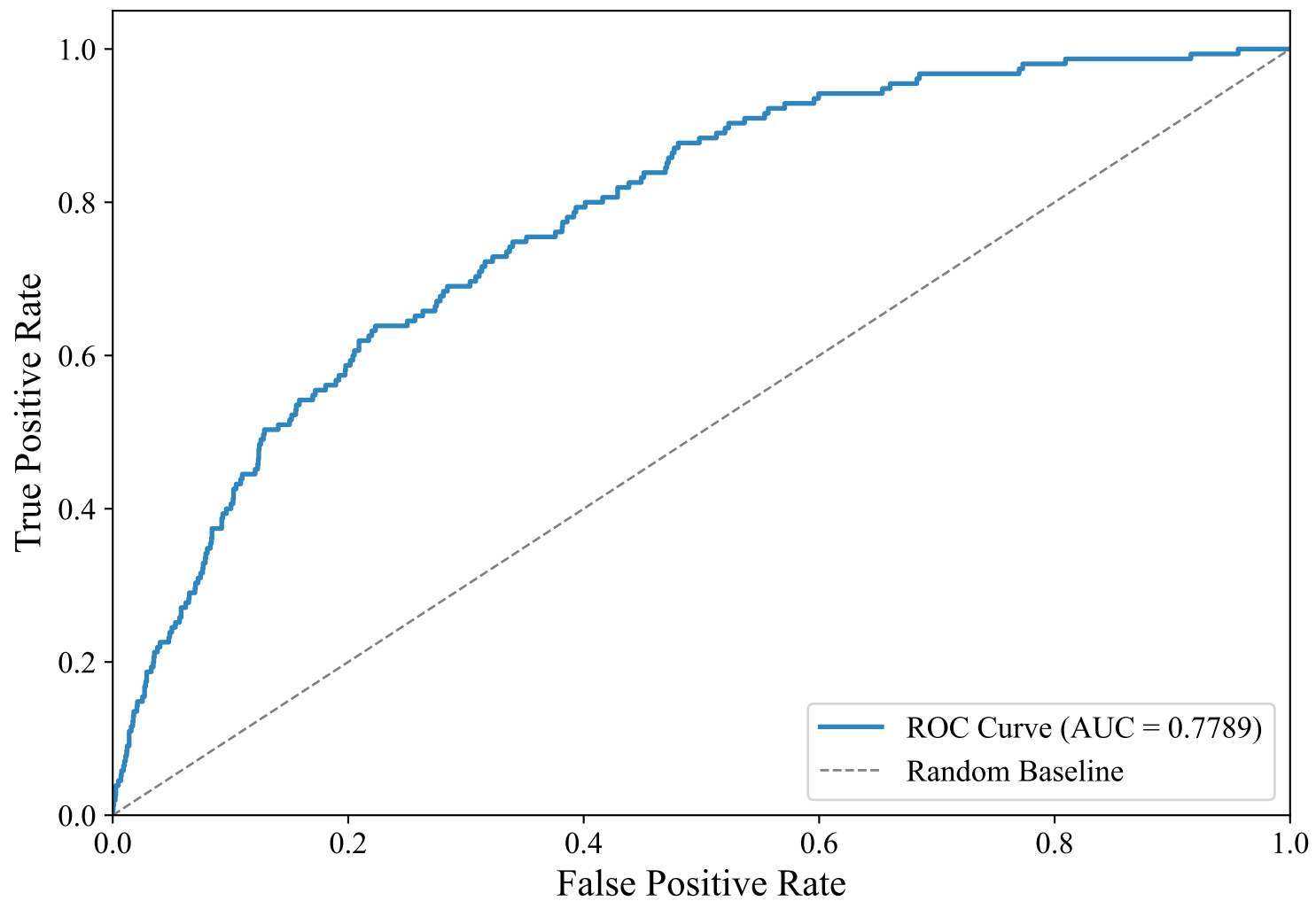
ROC Curve — SWEDISH_MANUAL (paraphrase-multilingual-MiniLM-L12-v2, XGBoost)
