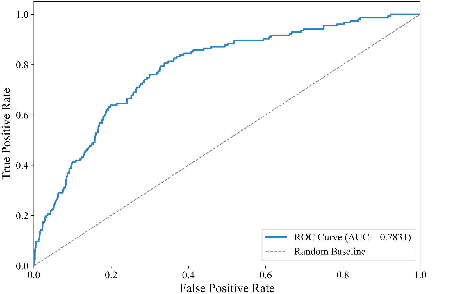
ROC Curve — SWEDISH_MANUAL (upskyy/bge-m3-korean, LightGBM)
