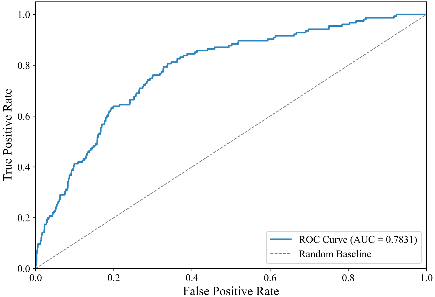
ROC Curve — SWEDISH_MANUAL (upskyy/bge-m3-korean, LightGBM_Optimized)
