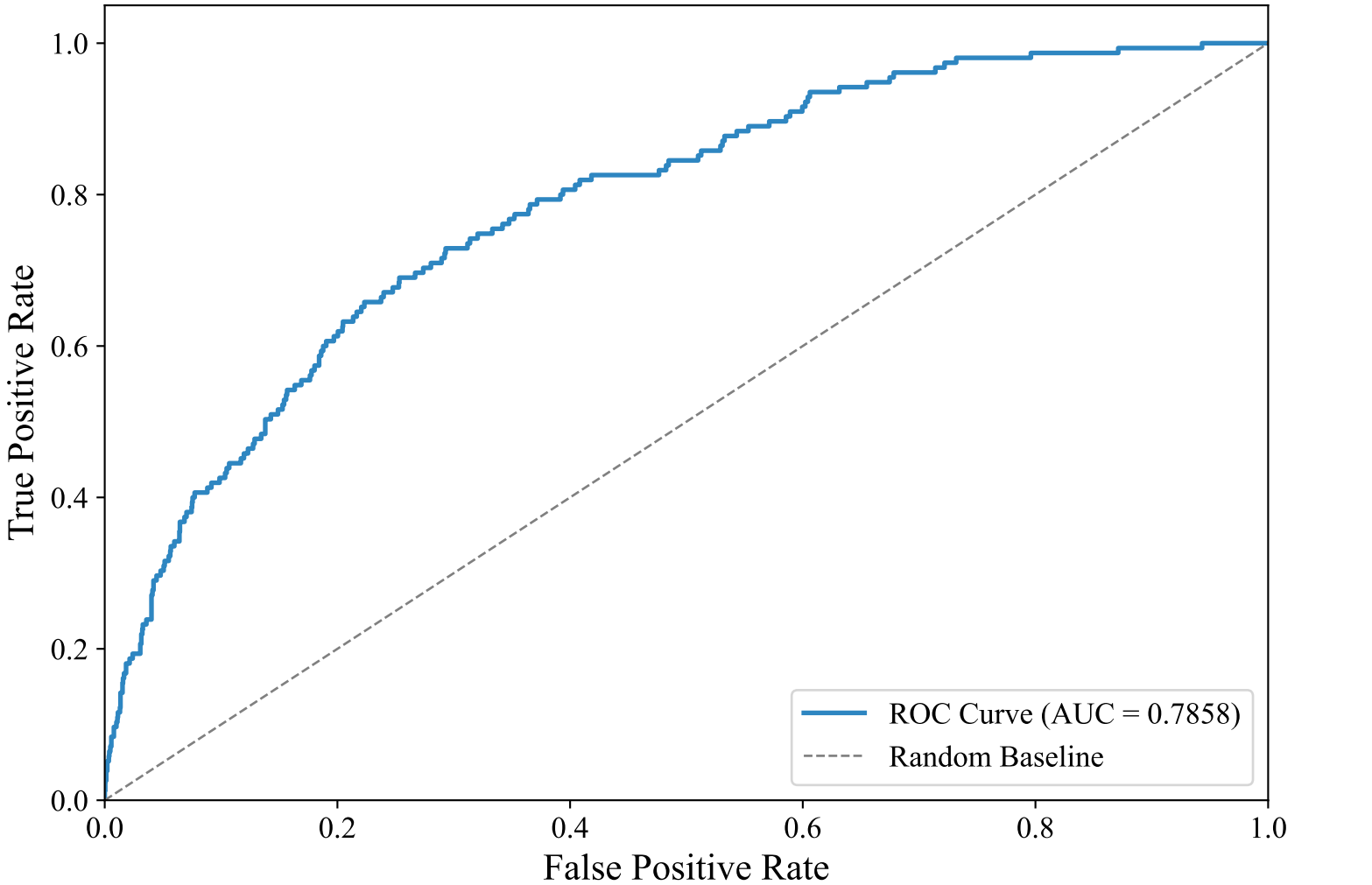
ROC Curve — SWEDISH_MANUAL (xlm-roberta-base, Voting_Ensemble)
