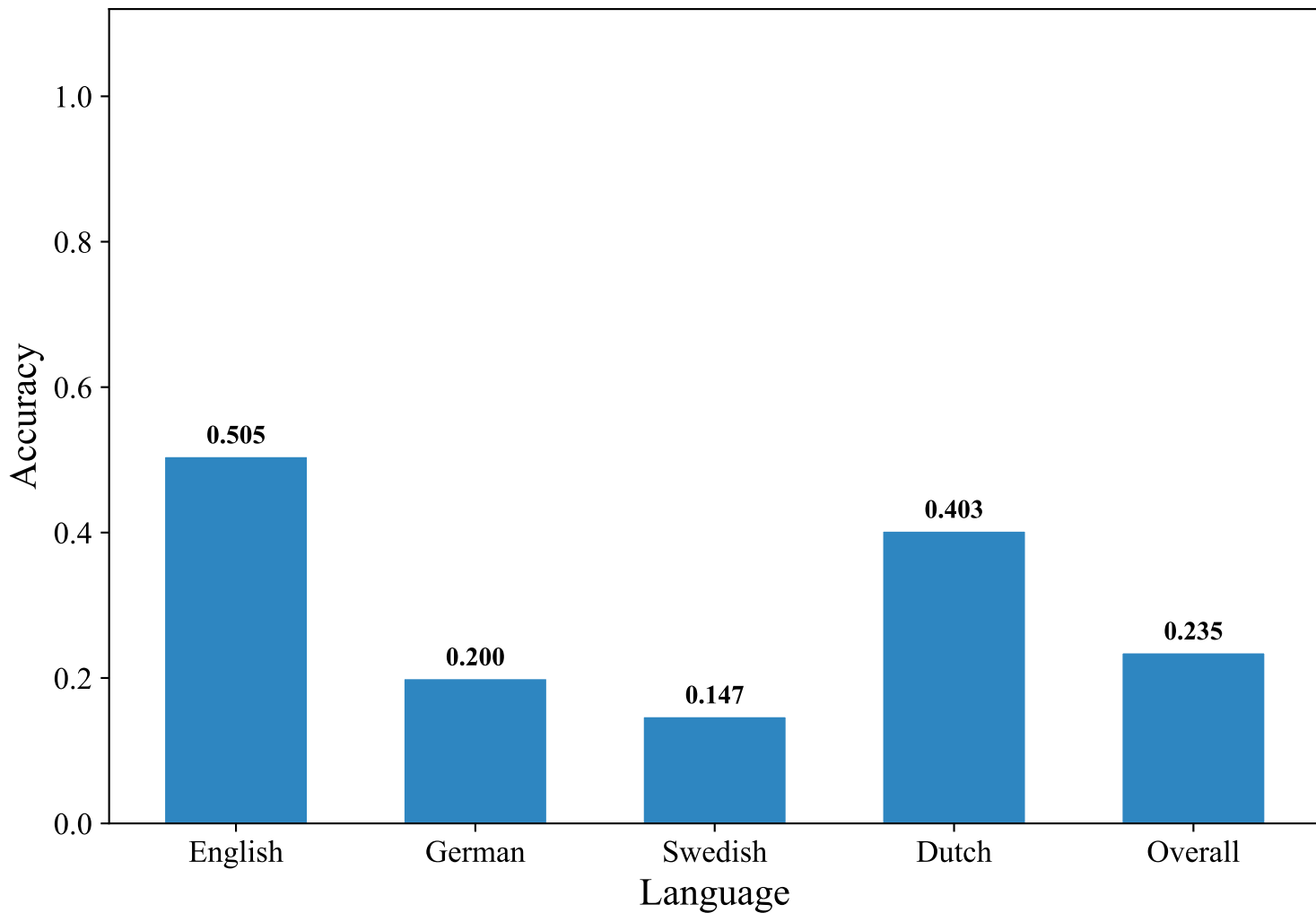
Iteration 7 — Accuracy by Language (XLM-RoBERTa XNLI)
