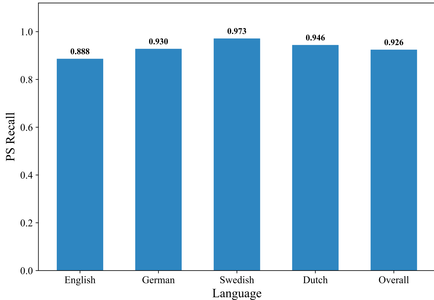
Iteration 7 — PS Recall by Language (XLM-RoBERTa XNLI)
