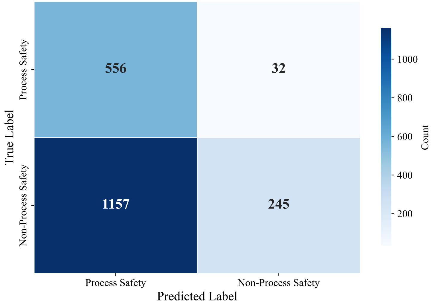
Confusion Matrix — Dutch (XLM-RoBERTa XNLI, Zero-Shot)
