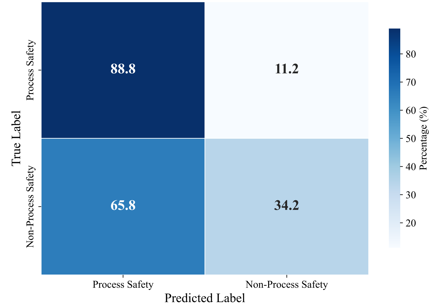
Normalised Confusion Matrix — English (XLM-RoBERTa XNLI)
