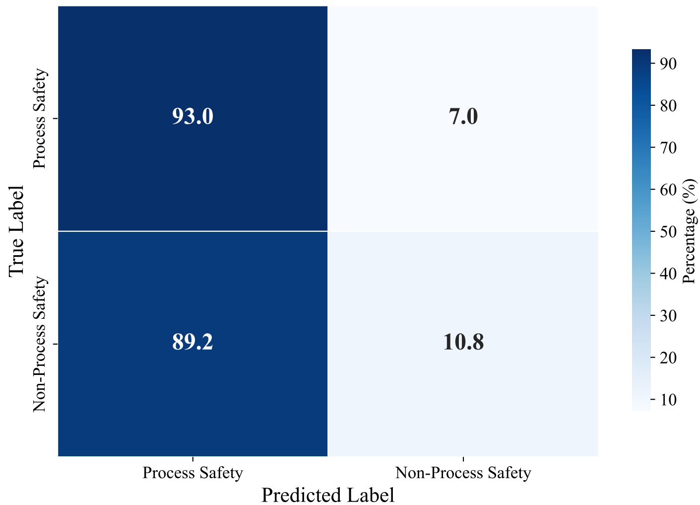
Normalised Confusion Matrix — German (XLM-RoBERTa XNLI)
