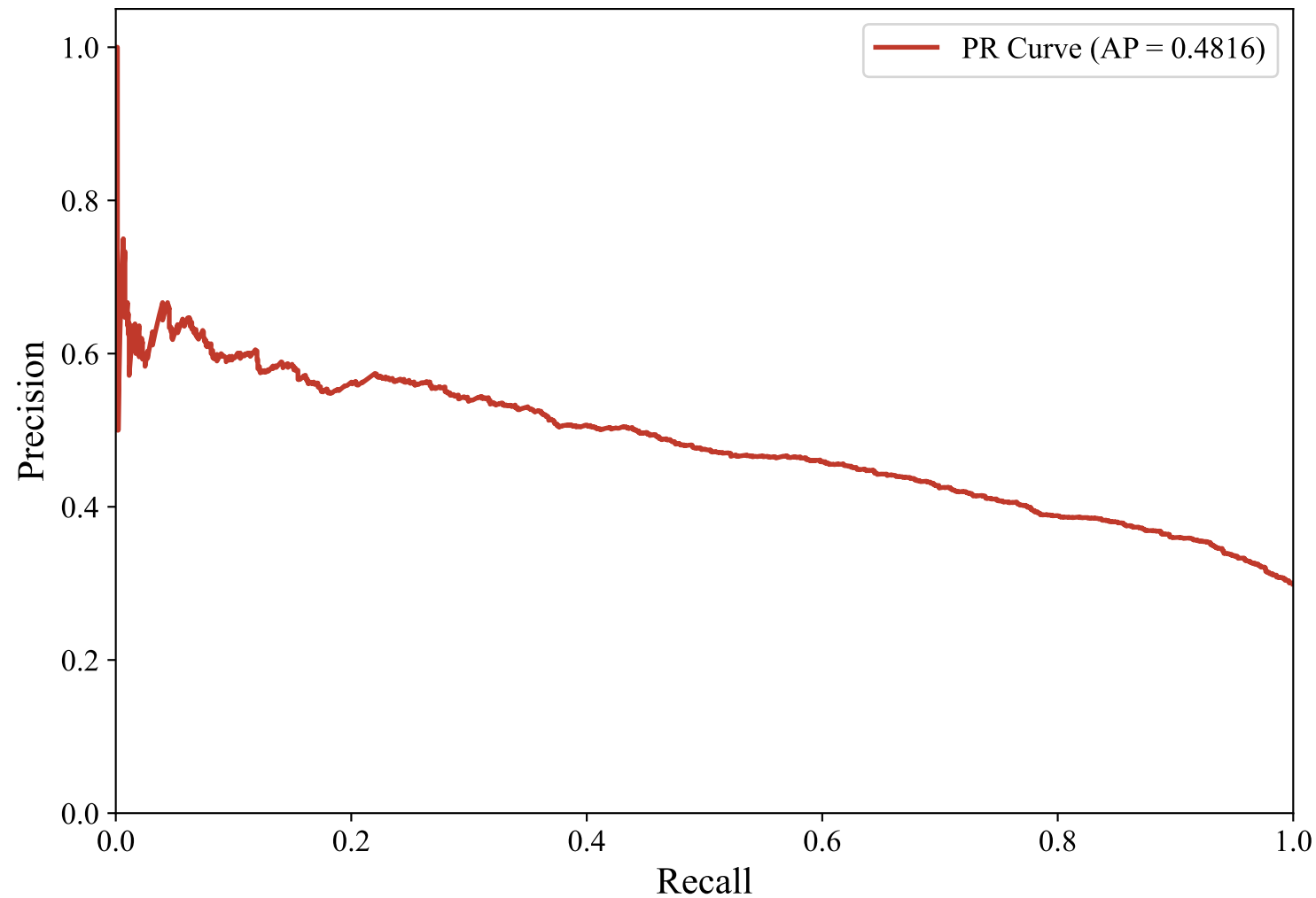
Precision-Recall Curve — English (XLM-RoBERTa XNLI, Zero-Shot)
