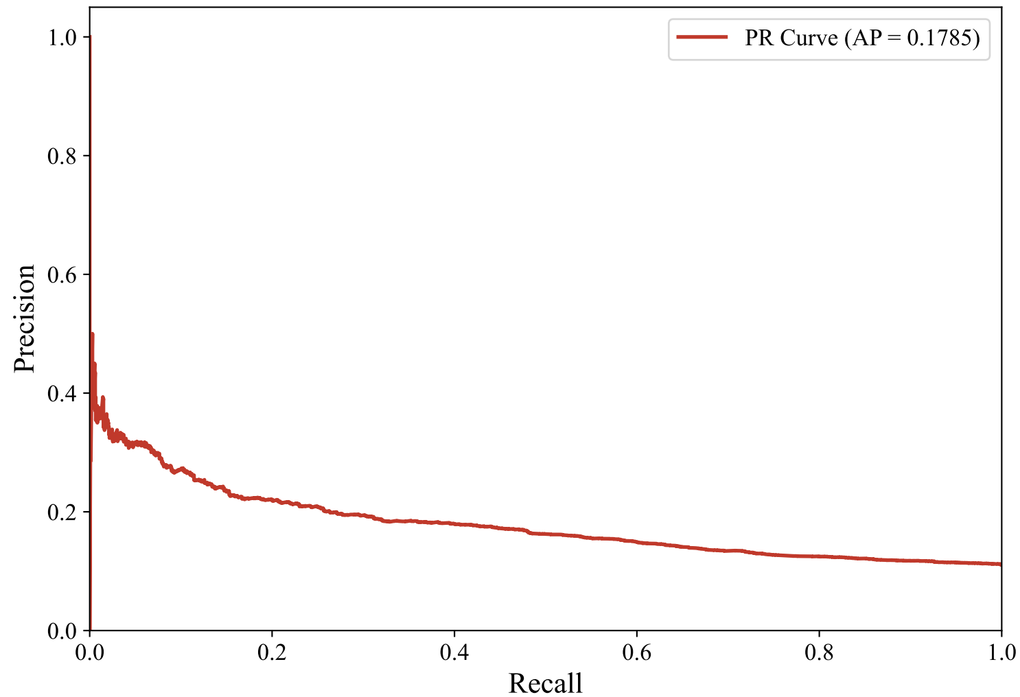
Precision-Recall Curve — German (XLM-RoBERTa XNLI, Zero-Shot)
