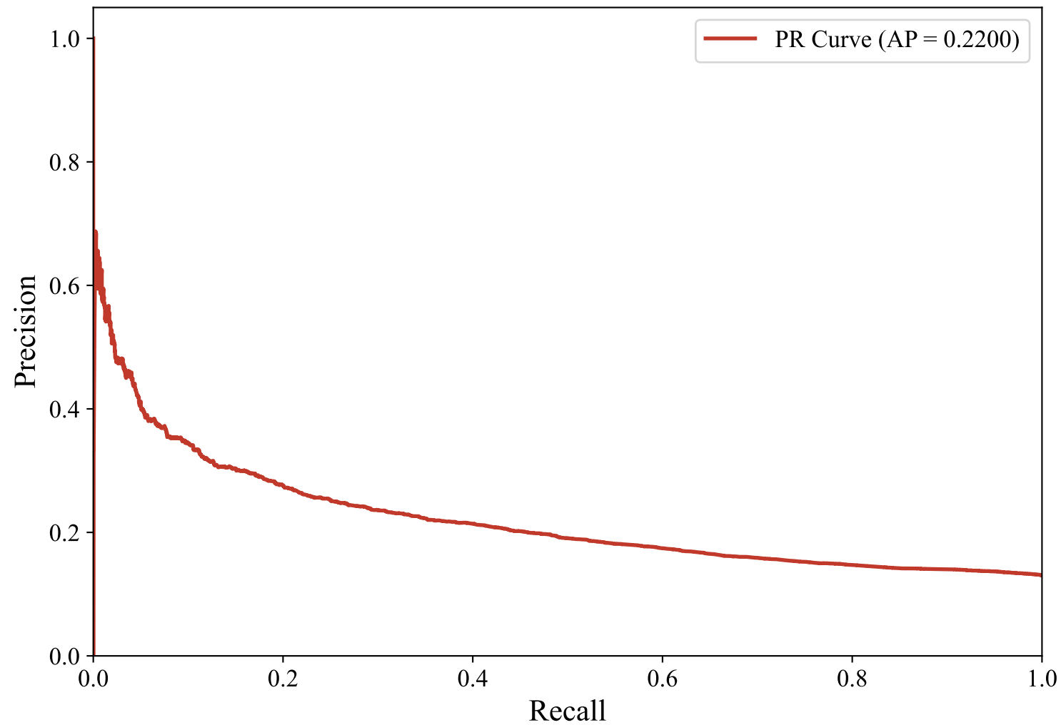
Precision-Recall Curve — Overall (XLM-RoBERTa XNLI, Zero-Shot)
