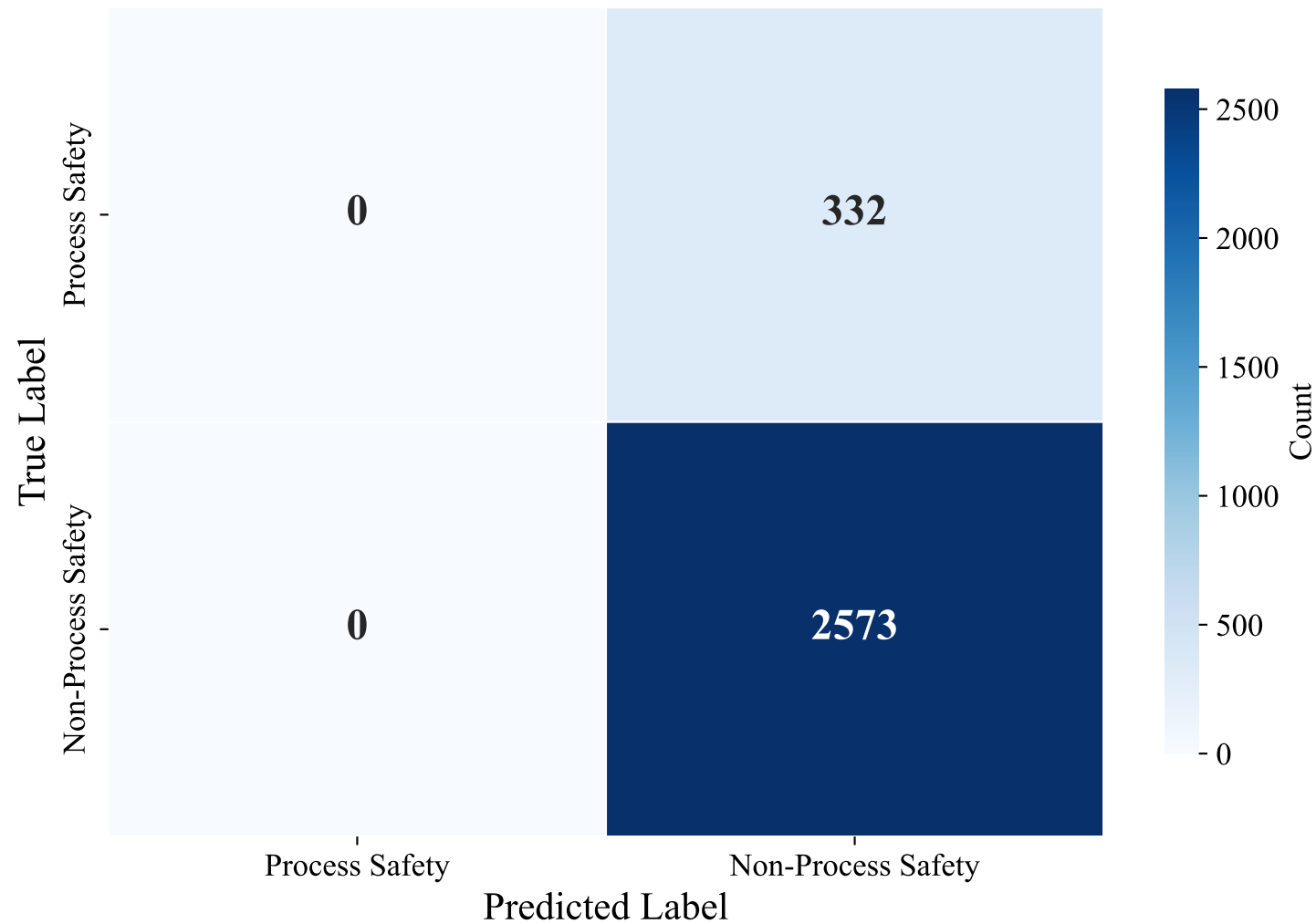
Confusion Matrix — German (flan-t5-large, Few-Shot)
