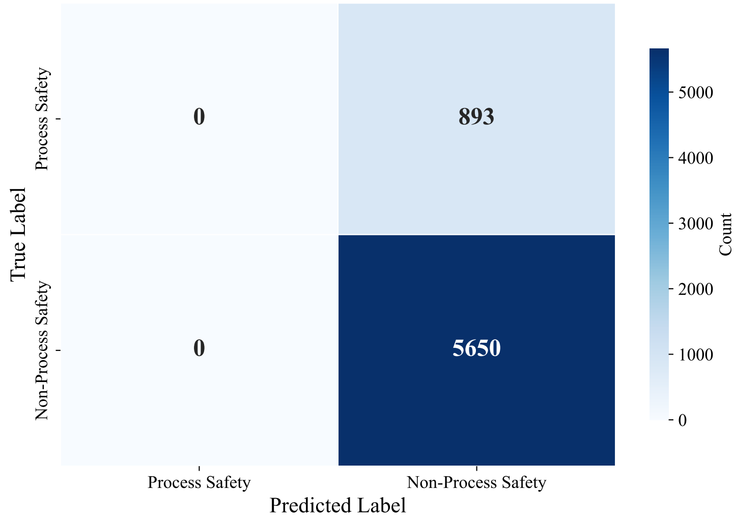
Confusion Matrix — Overall (flan-t5-large, Few-Shot)
