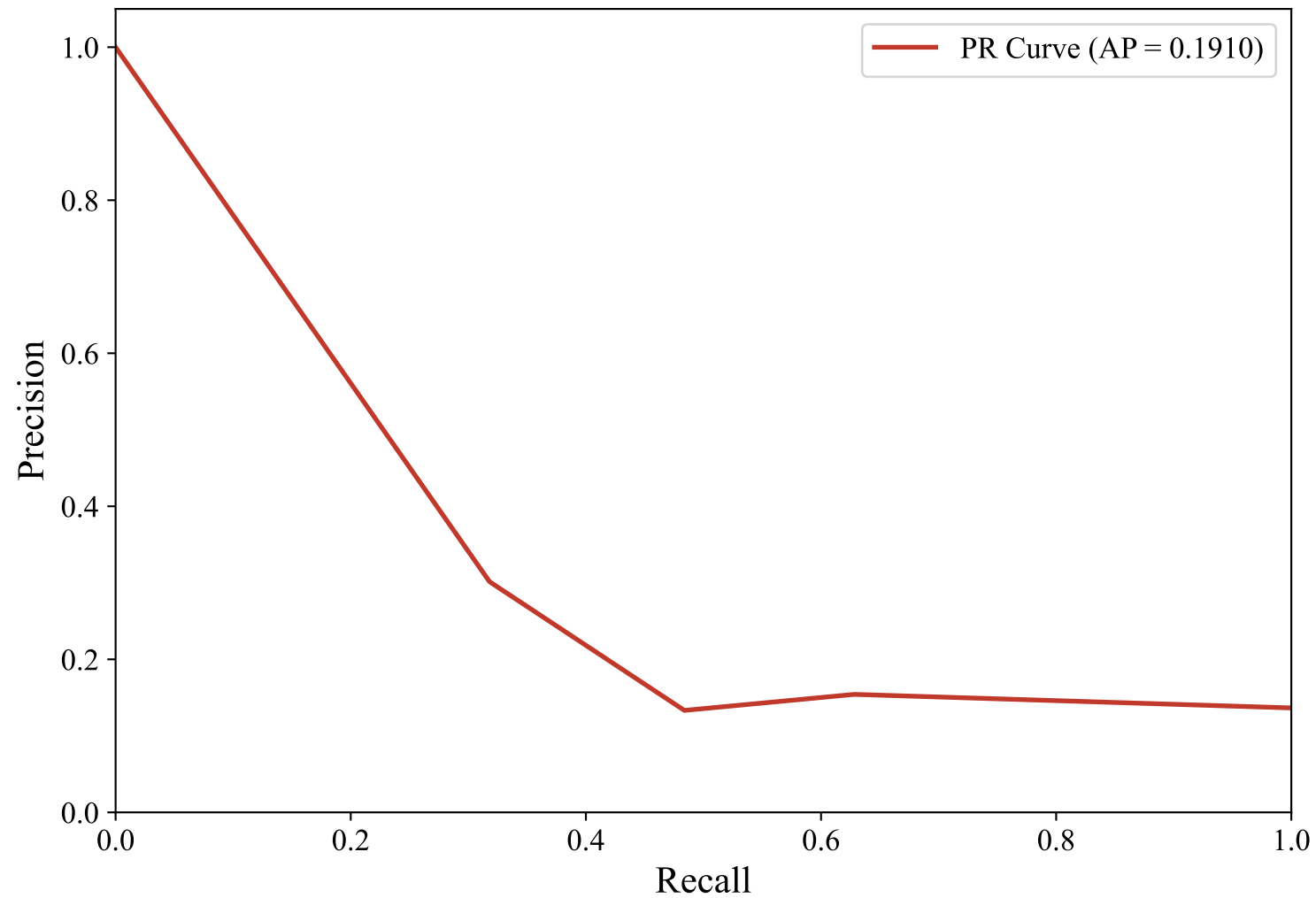
Precision-Recall Curve — Overall (flan-t5-large, Few-Shot)
