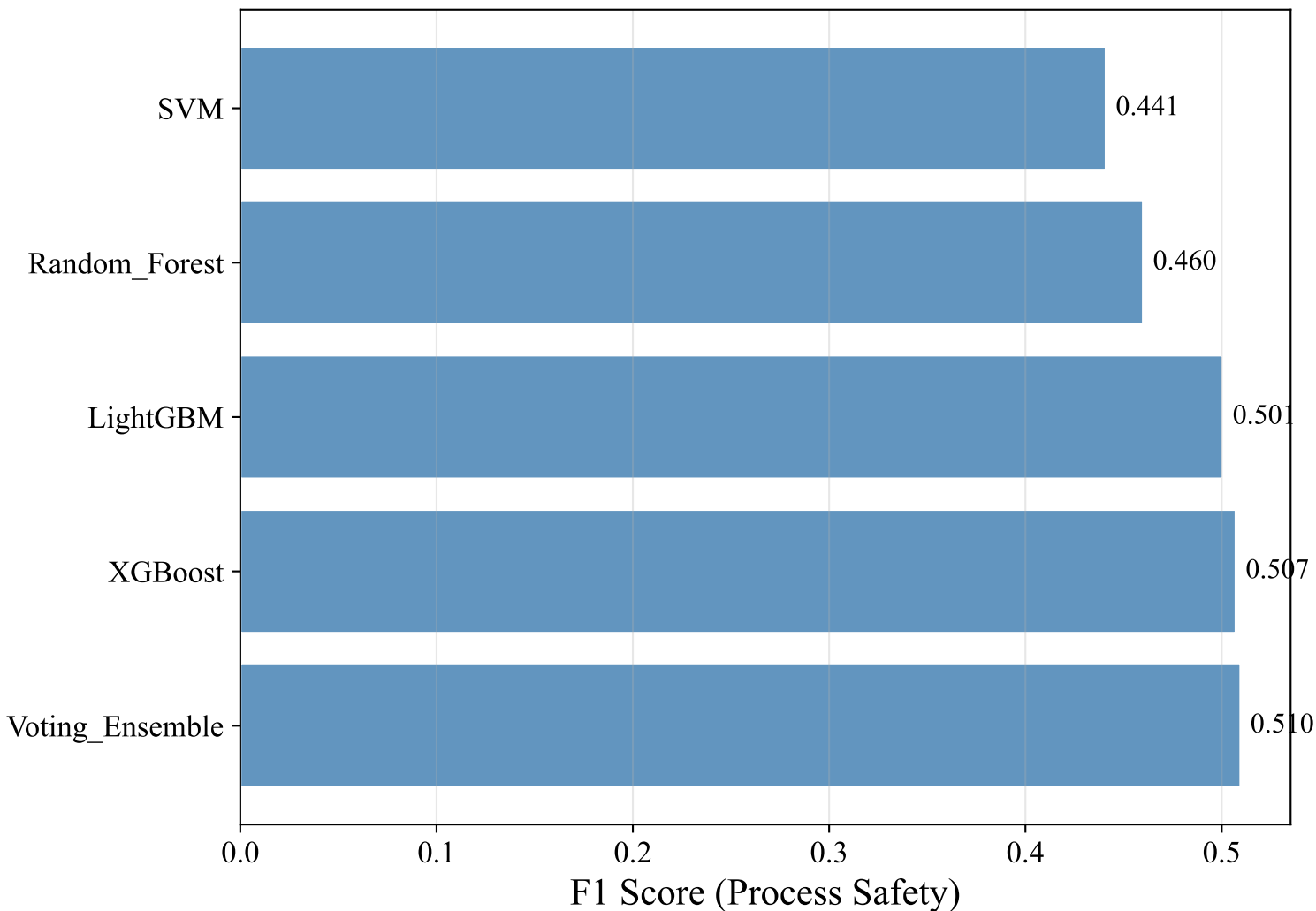
Average F1 Score by Classifier — Iteration 4
