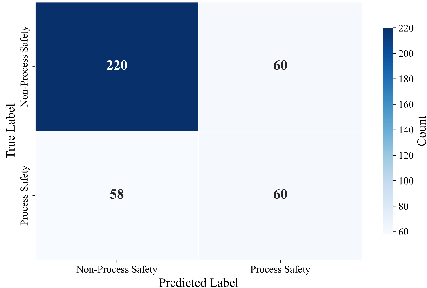
Confusion Matrix — DUTCH_MANUAL (intfloat/multilingual-e5-large-instruct, SVM)
