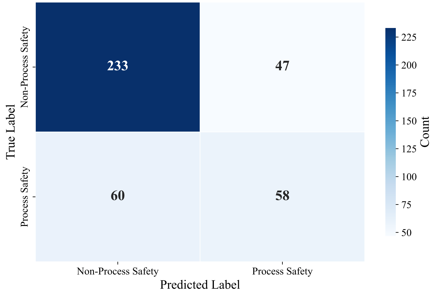
Confusion Matrix — DUTCH_MANUAL (paraphrase-multilingual-MiniLM-L12-v2, LightGBM)
