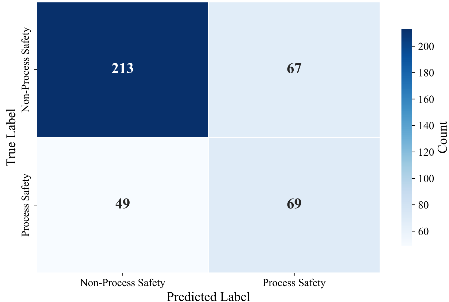
Confusion Matrix — DUTCH_MANUAL (paraphrase-multilingual-mpnet-base-v2, SVM)
