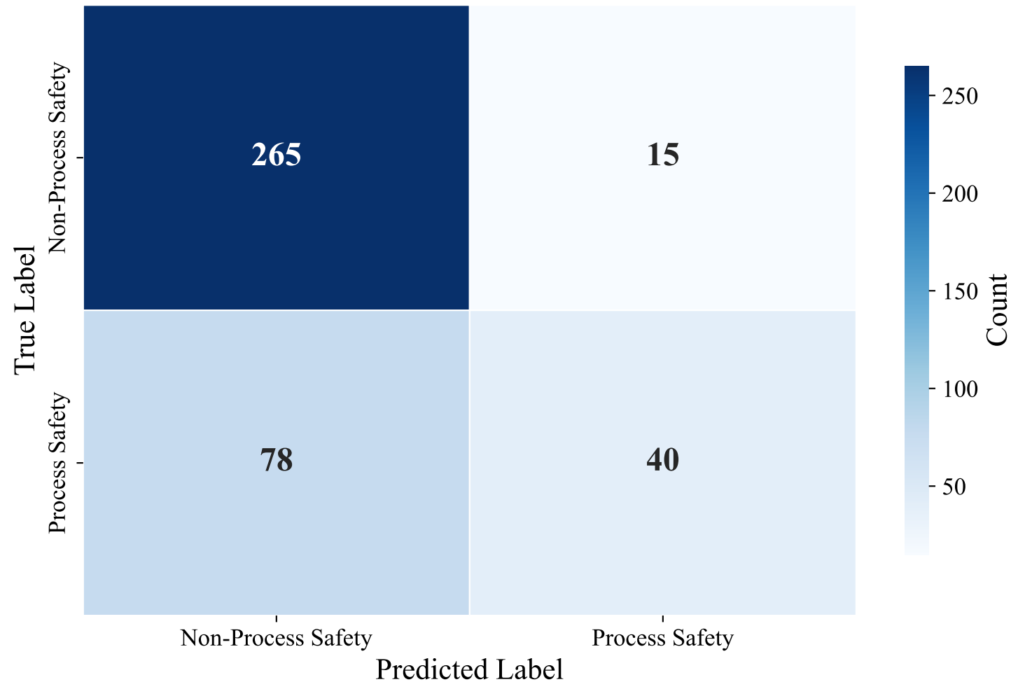
Confusion Matrix — DUTCH_MANUAL (snowflake-arctic-embed-l-v2.0, Random_Forest)
