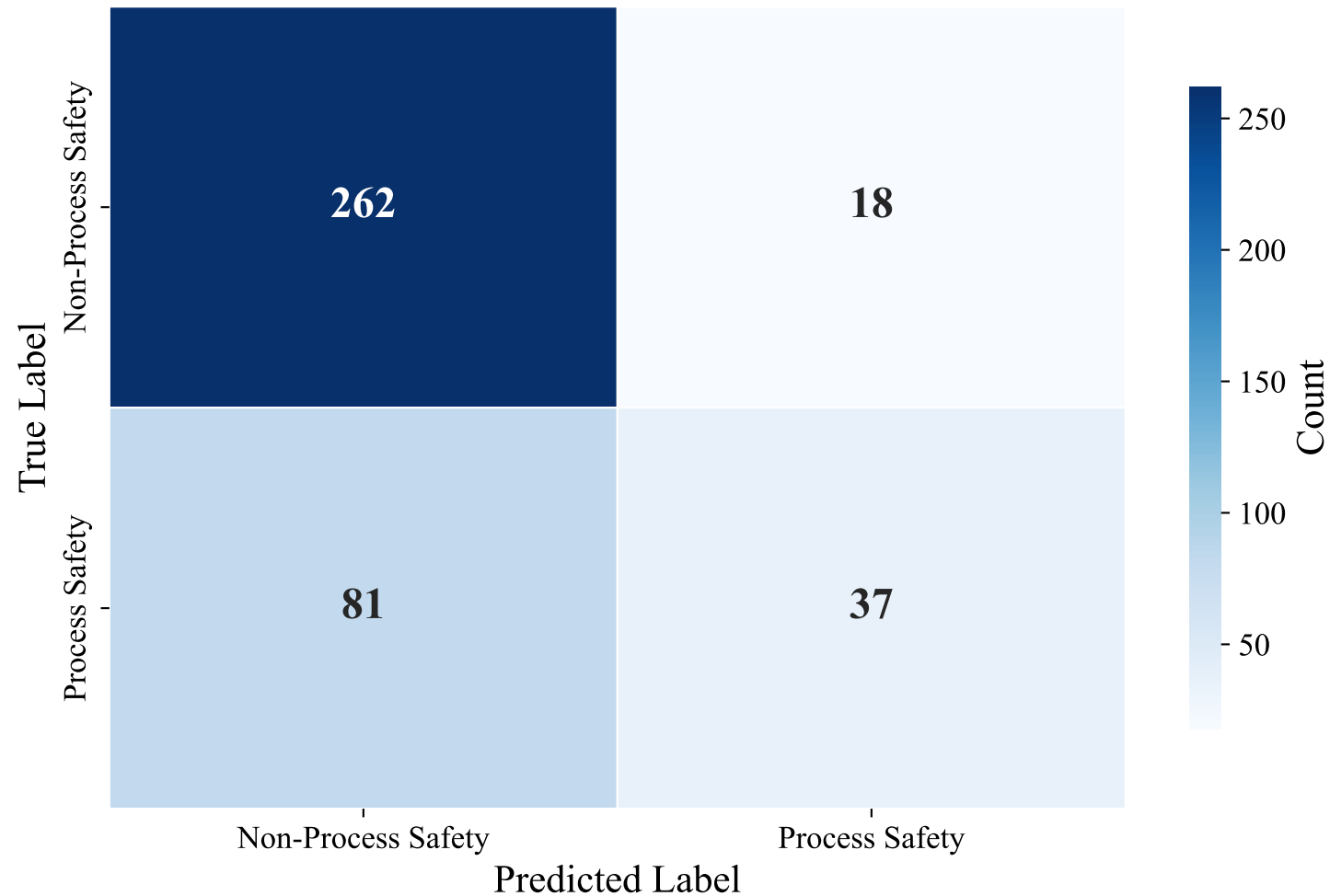
Confusion Matrix — DUTCH_MANUAL (upskyy/bge-m3-korean, Random_Forest)
