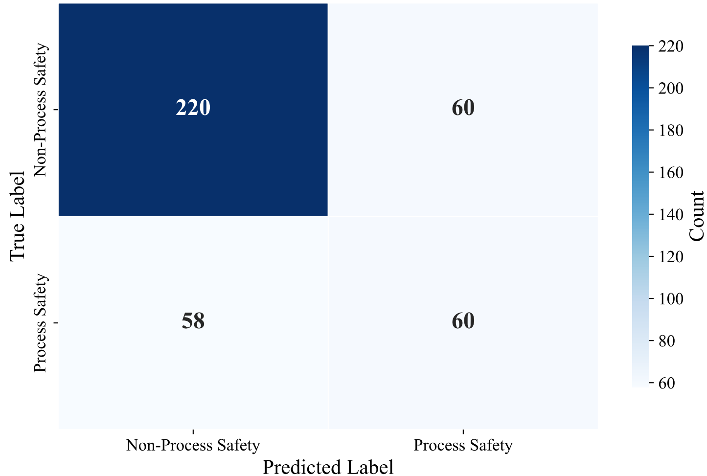
Confusion Matrix — DUTCH_MANUAL (upskyy/bge-m3-korean, SVM)
