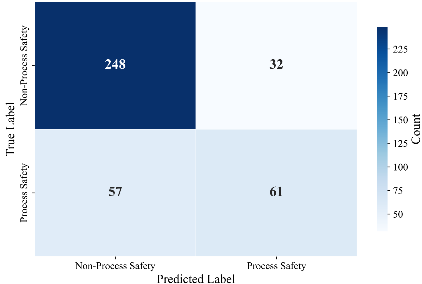
Confusion Matrix — DUTCH_MANUAL (xlm-roberta-base, LightGBM)
